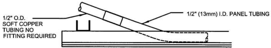
CONNECTION TO RADIANT PANEL TUBING (A)
